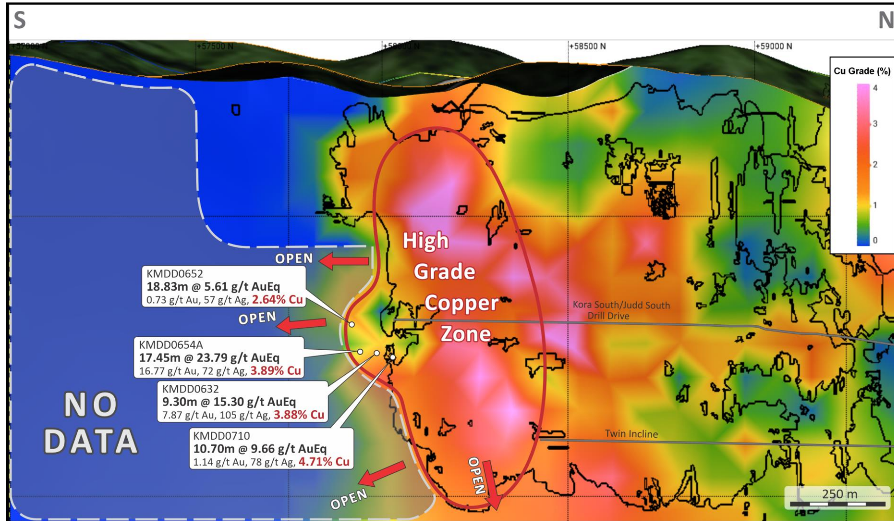
K2 Vein Copper Grade (%) Long-Section (Looking West) (1)
