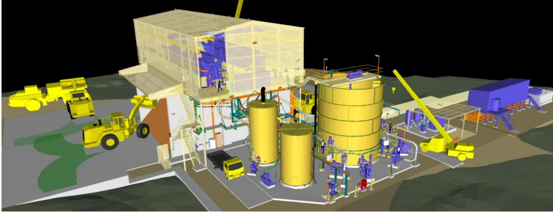
2. Surface Storage System Near Portal
