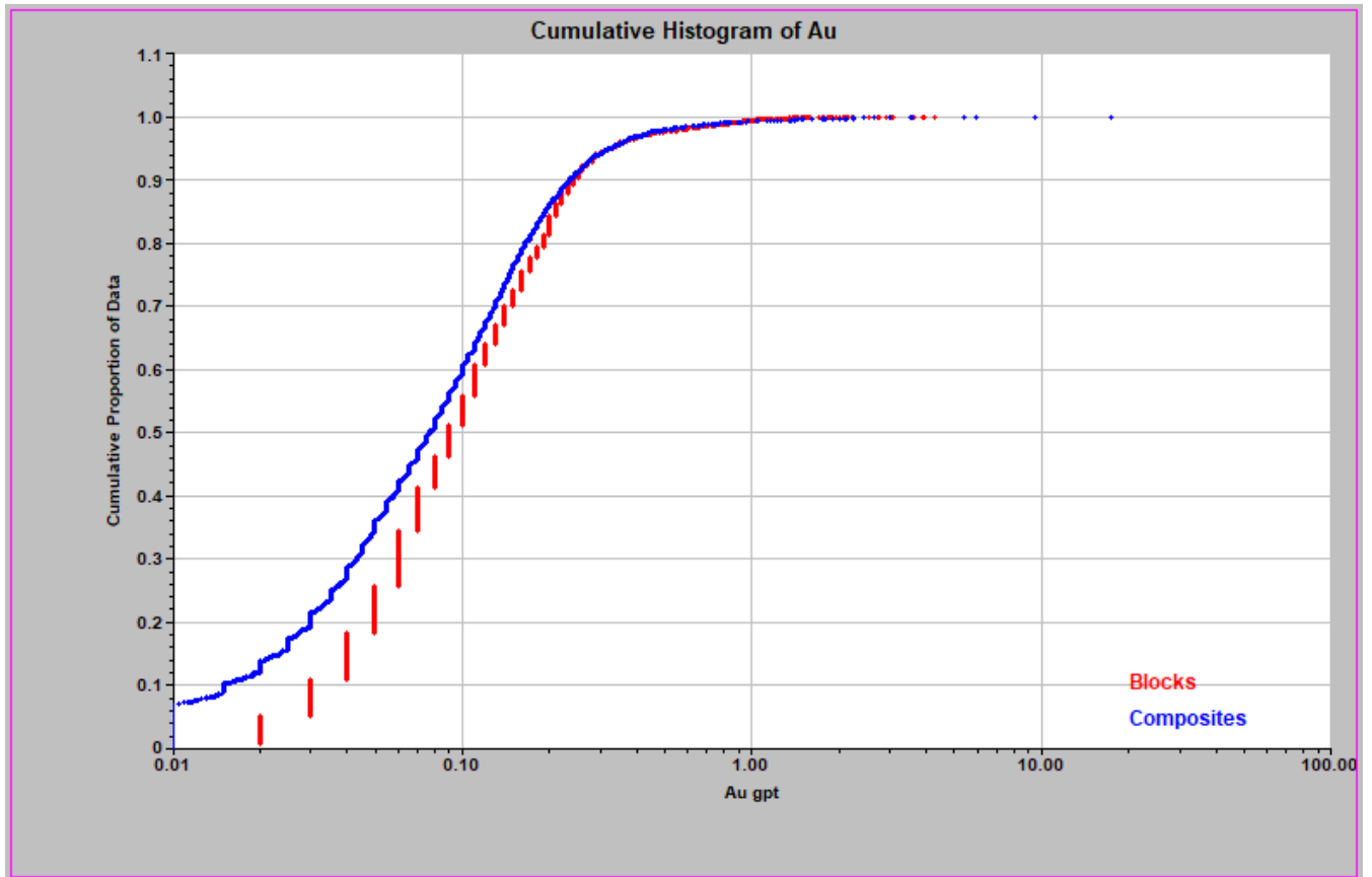
Figure 14-17. Cumulative Frequency Curves for Zone 2 Au Composite Values & Block Grades
