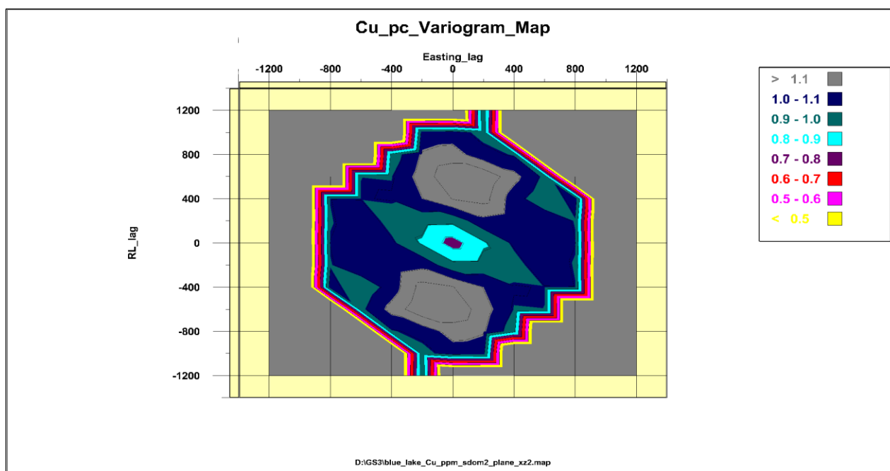
Figure 14-7. Cross Section (X-Z) Variogram Map for the Zone 2 Copper
