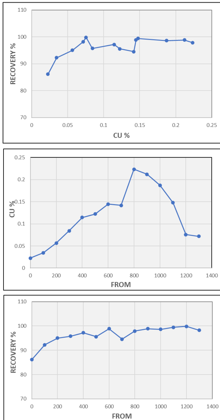
Figure 14-3. Grade v Core Recovery (top) / Cu Grade v Depth (mid) / Recovery v Depth (bot)
