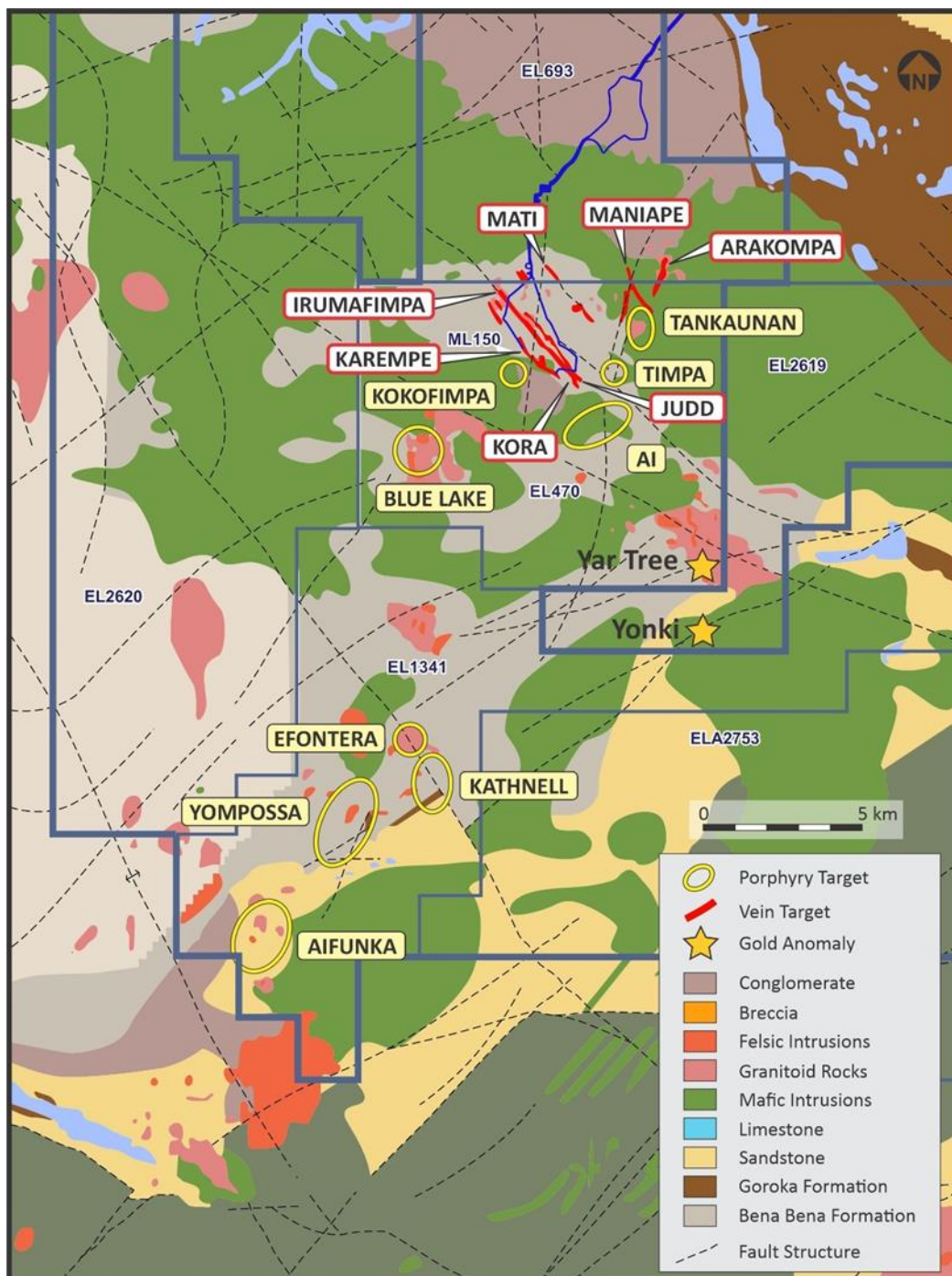
EL470 geology and known vein and porphyry prospects.
