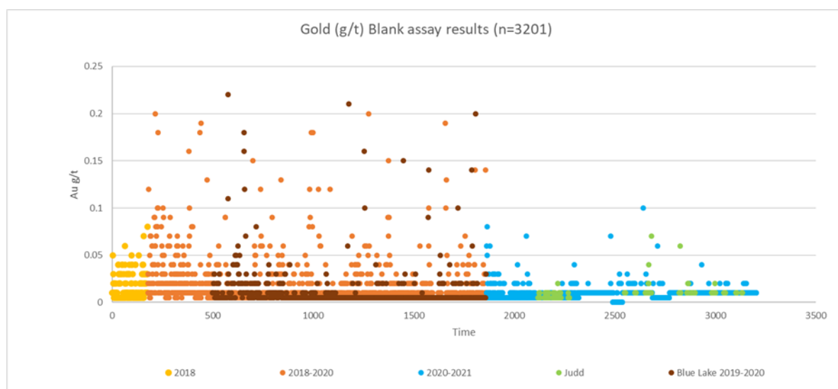
Figure 11-23. Gold blank results
