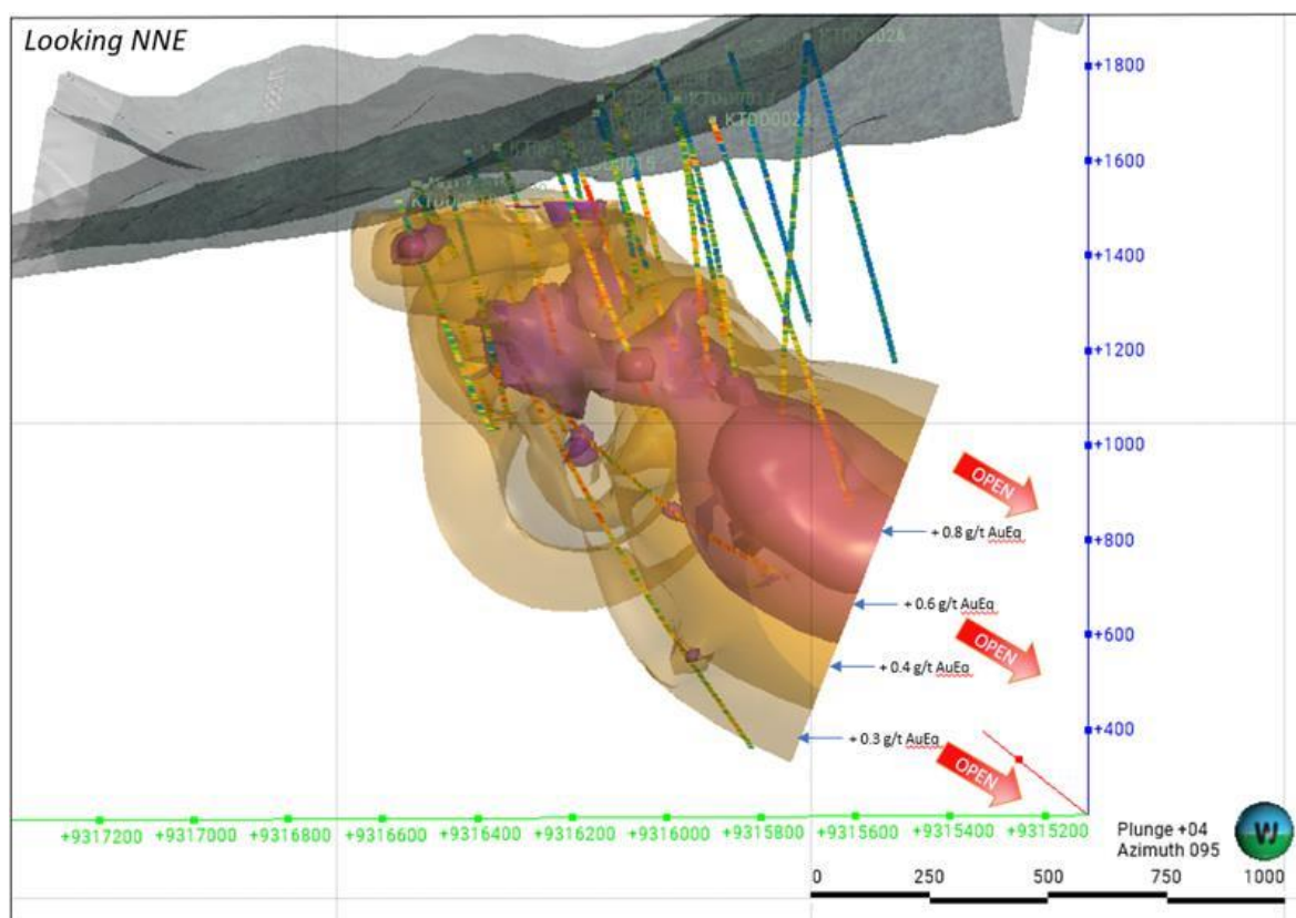
Figure 7-6. Blue Lake Porphyry – Section, viewed north-north-east Drill holes showing downhole gold and copper grades and distribution of mineralization Source: K92ML (2022)
