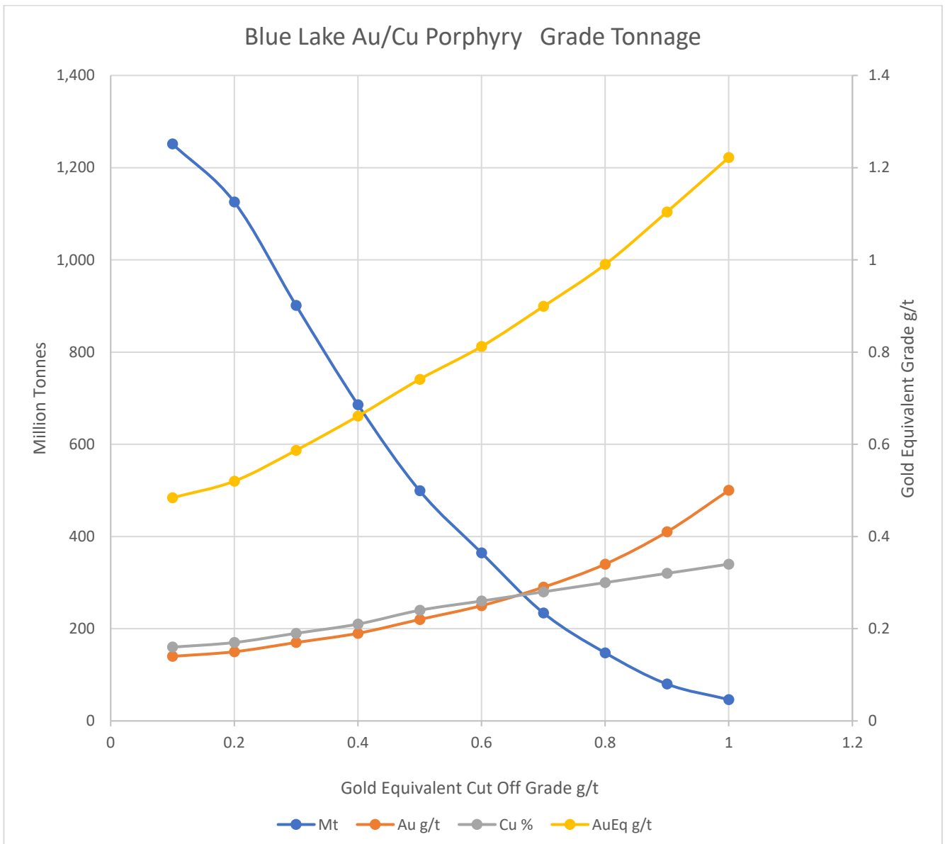
Figure 14-13. Blue Lake Porphyry Grade-Tonnage Curves
