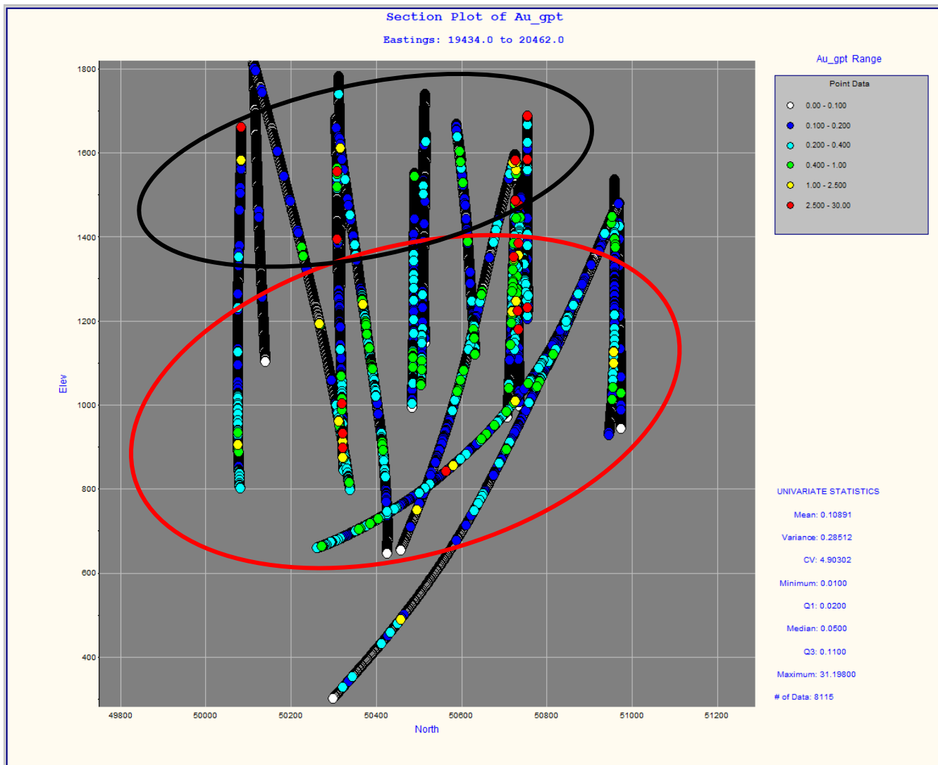
Figure 14-2. Long Section with 2m Gold Composites, looking West (zoom for better resolution)
